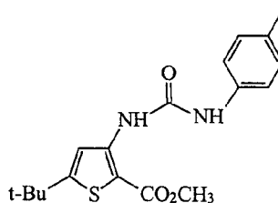
5-tert-Butyl-3-(3-p-tolyl-ureido)-thiophene-2-carboxylic acid methyl ester
